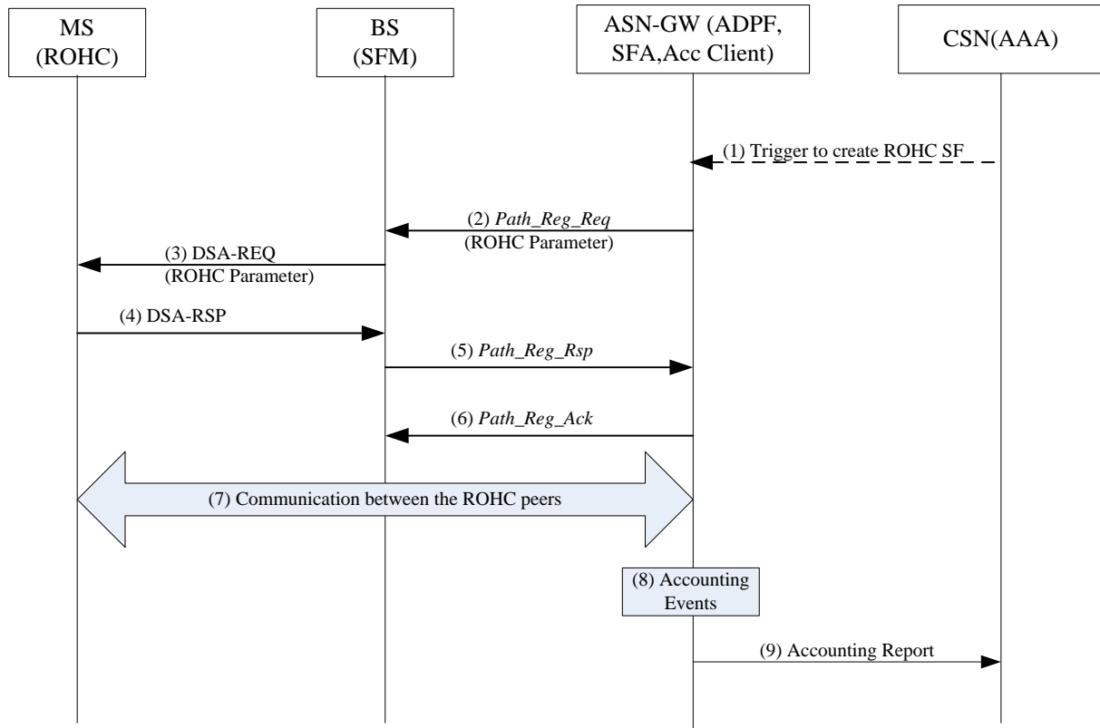
2 Figure 6-8 The accounting Procedure for ROHC SF
