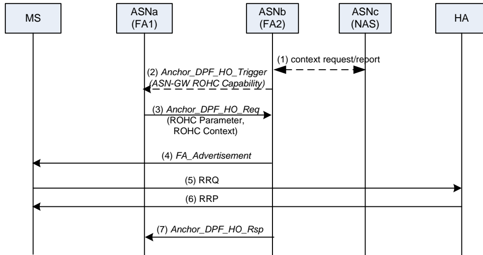
10 Figure 6-6 ROHC Relocation (CMIPv4)
