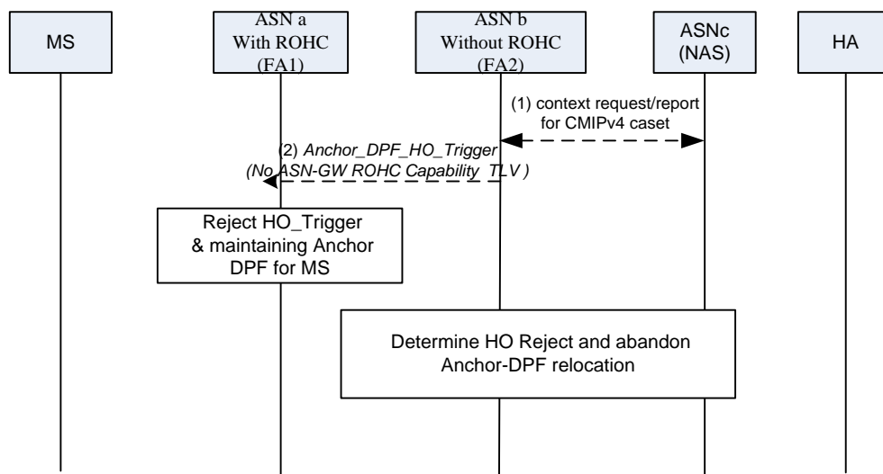
27 Figure 6-7 ROHC Relocation (Failure)
