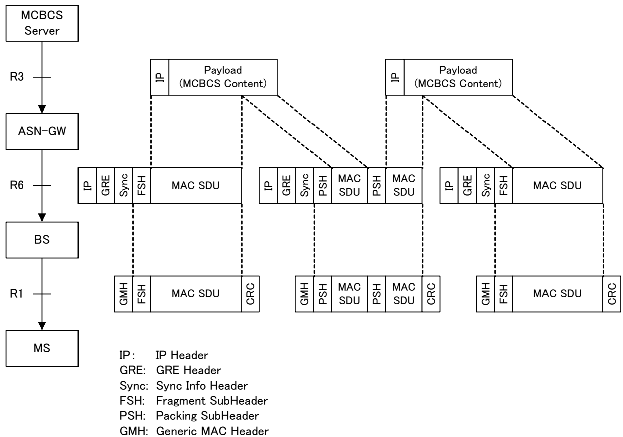
Figure 3-3 - Type-4 MCBCS Data Transfer
