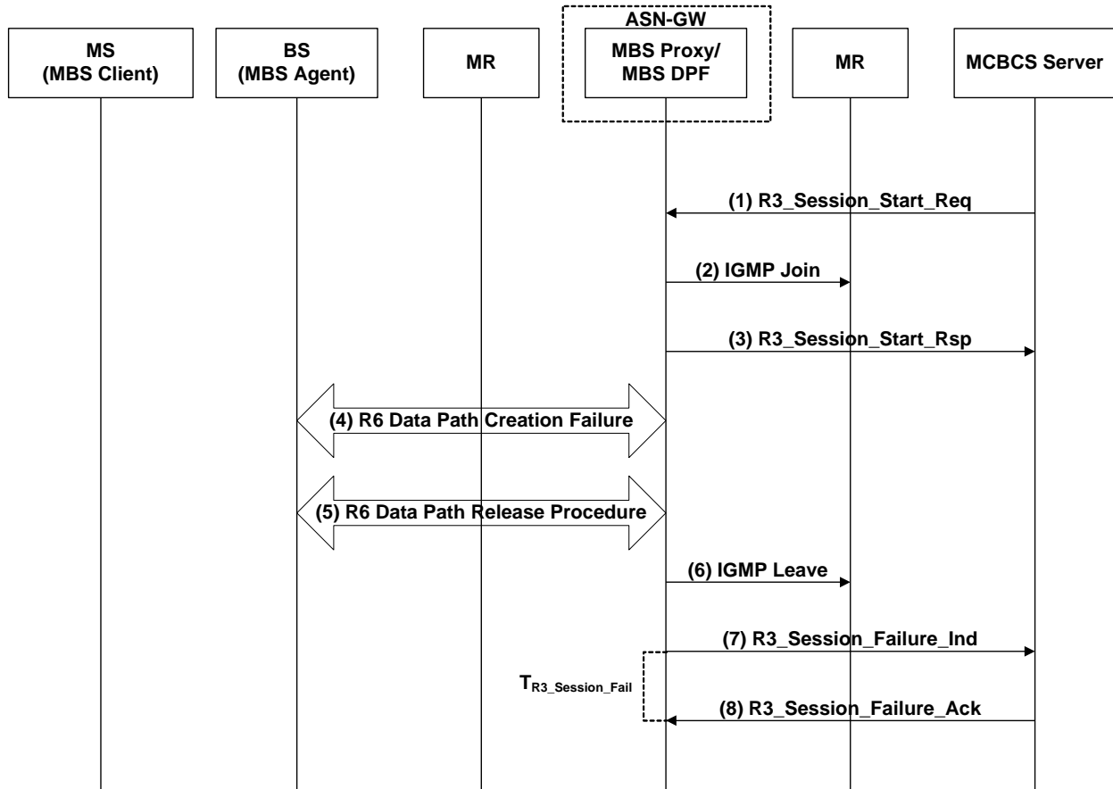
6 Figure 4-7 - MCBCS Data Path Creation Failure under All BSs
