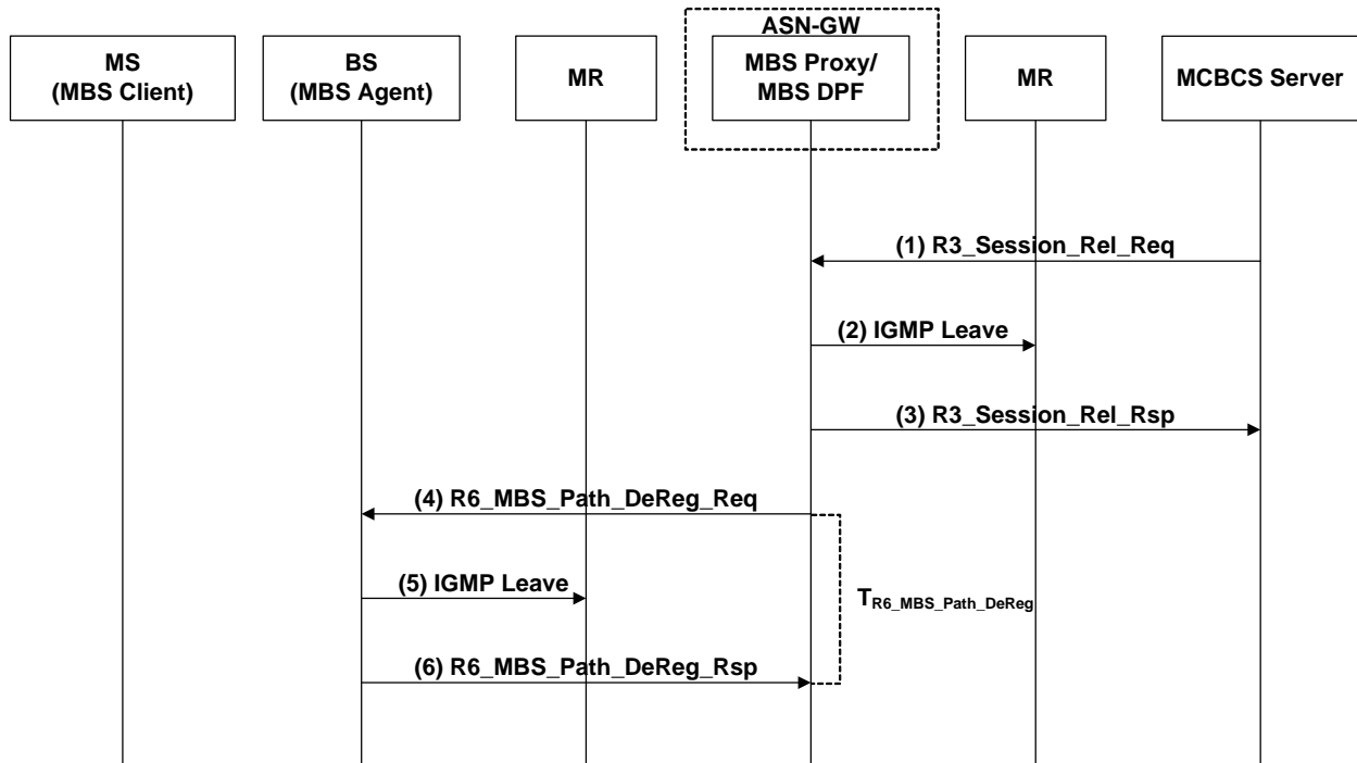
12 Figure 4-8 - MCBCS Data Path Release Procedure
