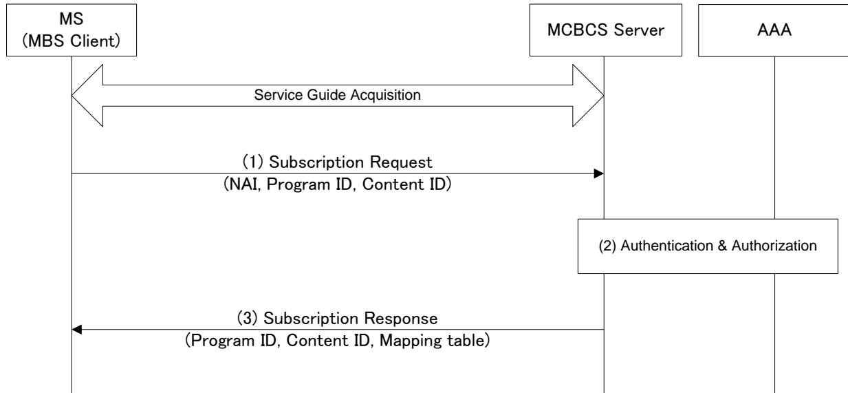
10 Figure 4-3 - Online Subscription Procedure
