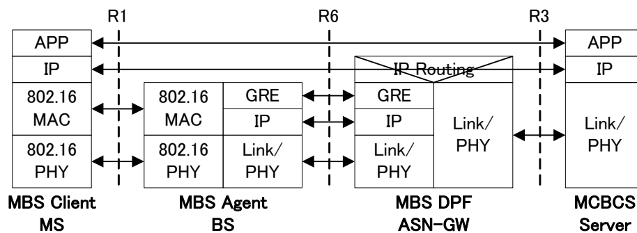
15 Figure 3-2 - Protocol Stack for Type-4 MCBCS Data Plane
