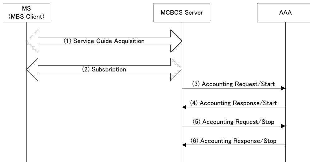
22 Figure 4-11 - Call Flow for Subscription Based Accounting
