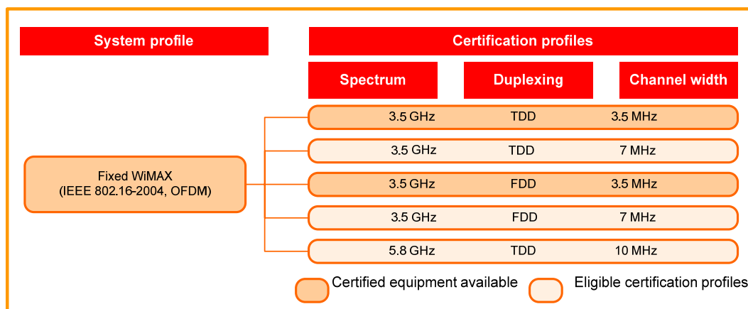
Figure 3. System and certification profiles
